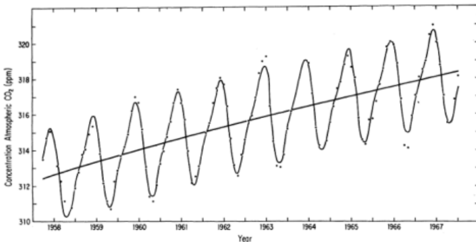
FIG. 5. Long-term variations in the concentration of atmospheric CO 2 at Mauna Loa Observatory. The dots indicate the observed monthly average concentrations. The oscillating curve is a least squares fit of these averages based on an empirical equation containing 6 and 12 month cyclic terms and a trend function. The slowly rising curve is a plot of the trend function, chosen to contain powers of time up to the third.
